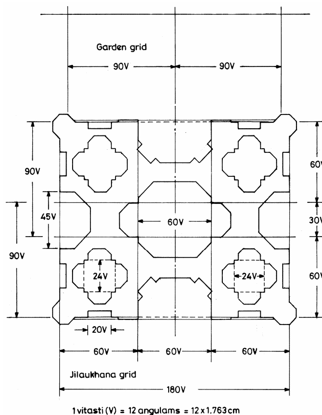
Figure 4. Proposed novel modular plan and predicted dimensions of the main gate between jilaukhana and charbag sections based on modular grid of 60V. The vitasti (V) equals 12 angulams and each angulam measures 1.763 cm.
