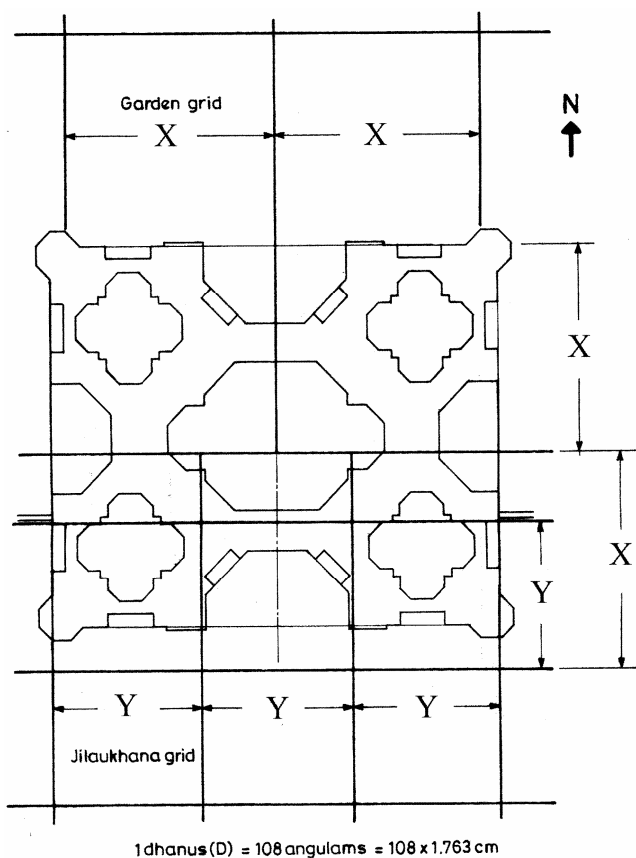
Figure 3. Modular plan of the main gate separating the jilaukhana from the charbag based on the modular grid design of Barraud 6 . The striking lack of symmetry in the modular plan must be noted. In this figure, the 23-gaz unit is referred to as X and the 17-gaz unit as Y.
